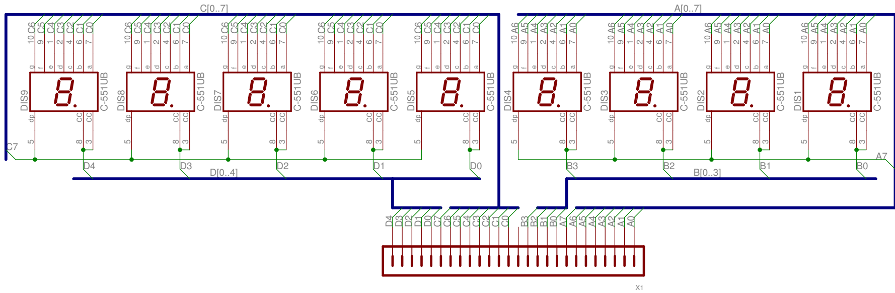
Frequency Counter - LED Display Module Gaspar Sinai, Tokyo, 2012-04-22
